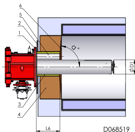
Low NOx burner LN30 (Standard mounting)
